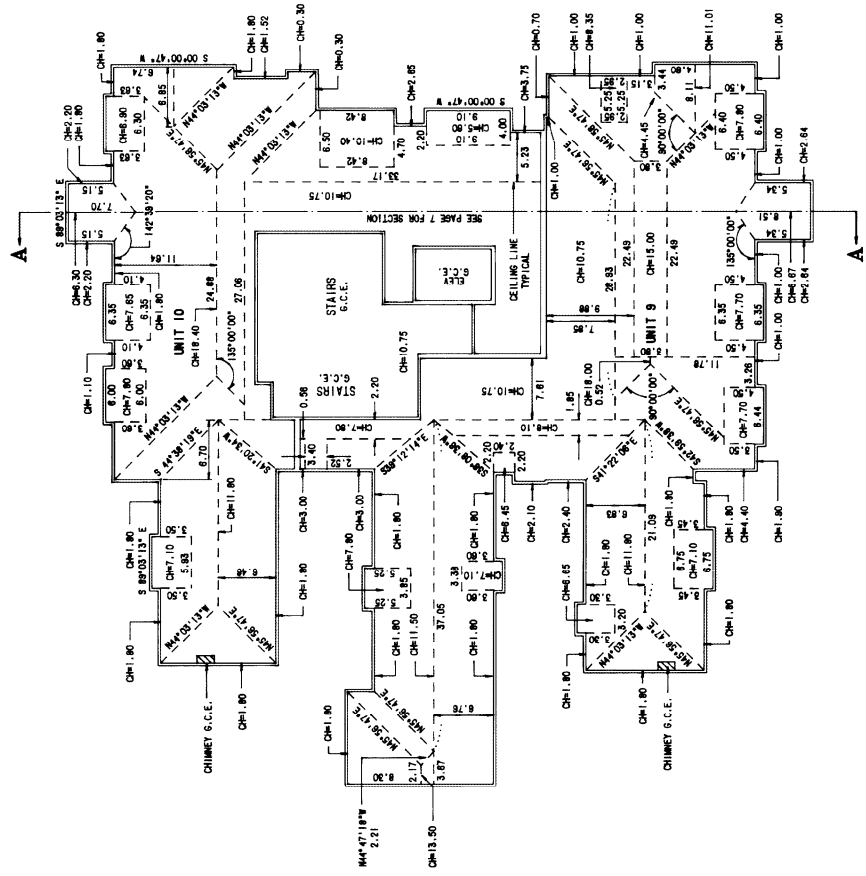
THIRD FLOOR - CEILING
